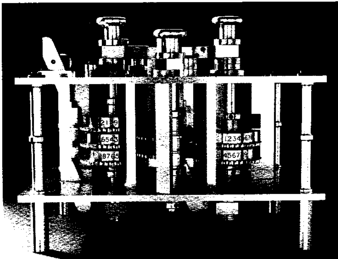
Portion of Charles Babbage's Difference Engine No. 2. View of the trial piece of Babbage's DE2 built by the Science Museum. The portion shown was built by the Science Museum to Babbage's original designs as a trial piece to verify the basic logic and construction of the calculating mechanism. The trial piece measures 17 inches by 11.75 inches by 13.5 inches. It adds a two-digit number to a two-digit number, taking account of any carry. It is the first physical realization of any part of the engine. (Science Museum photograph)
